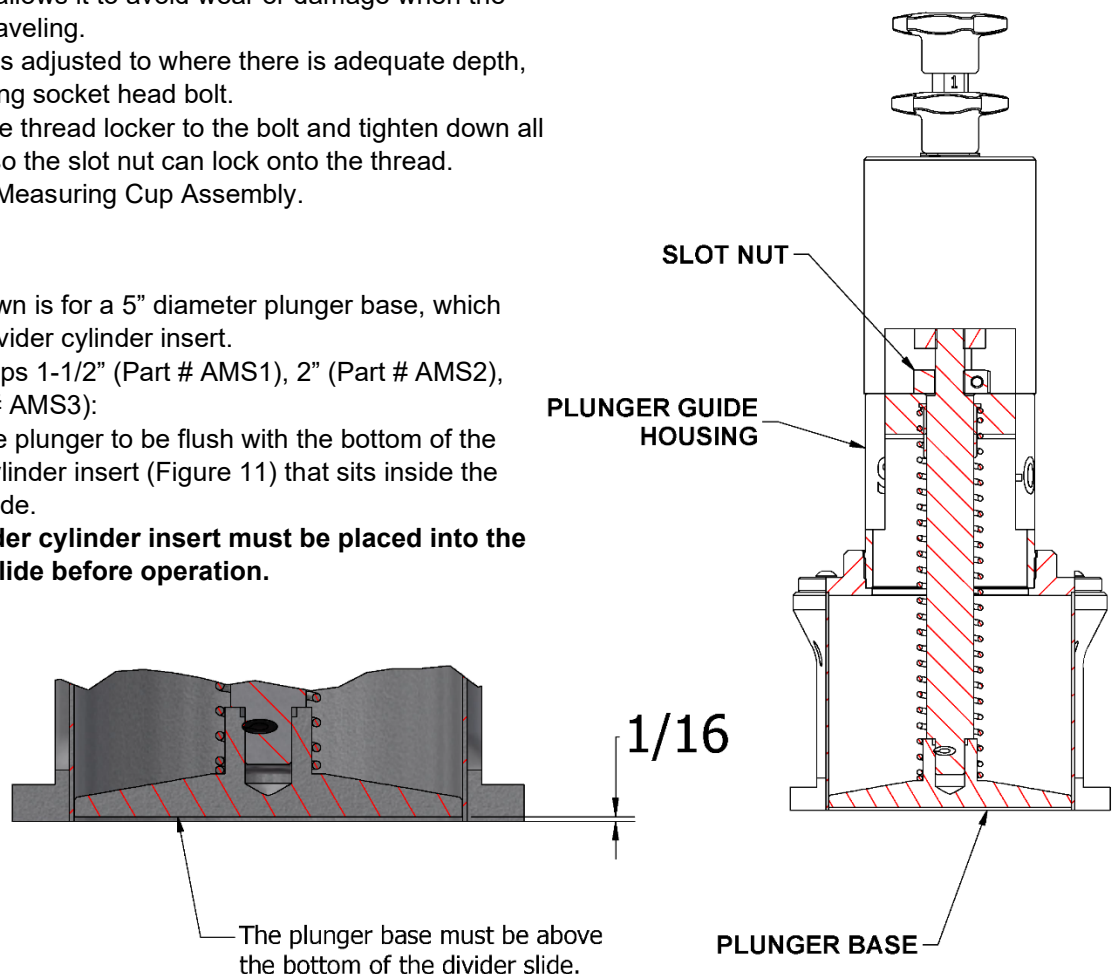
Figure 12: Measuring Cup Depth
