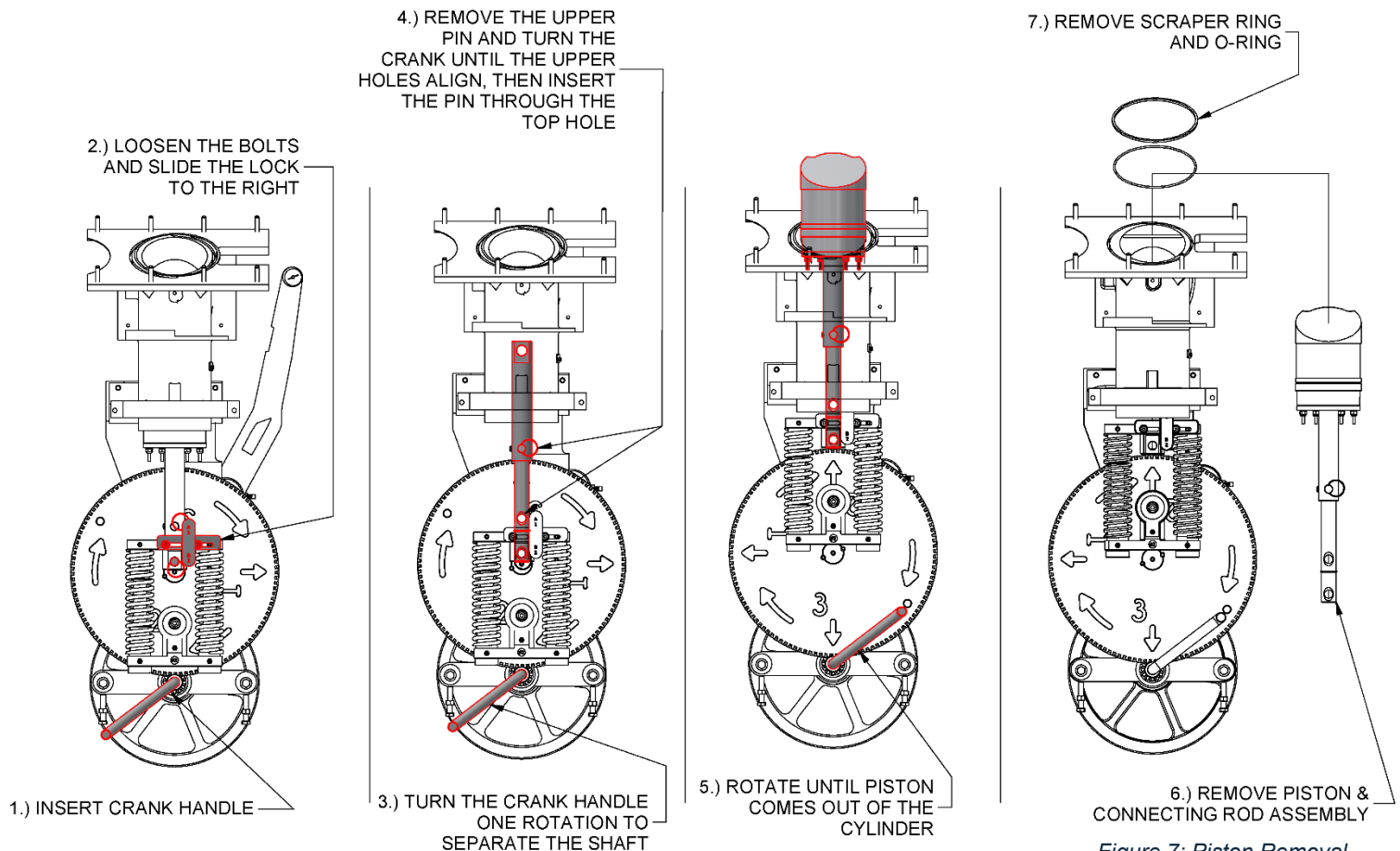
Figure 7: Piston Removal
