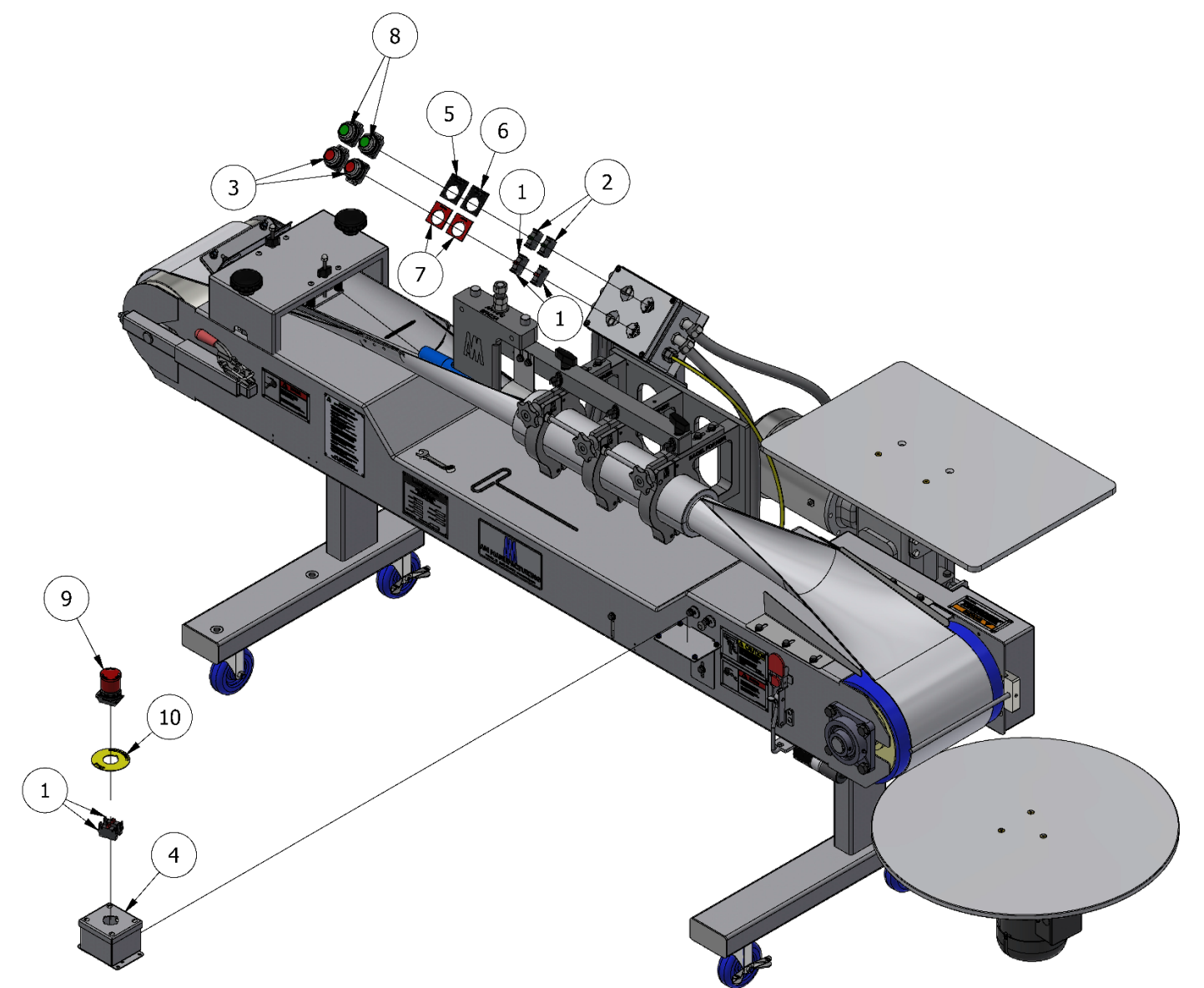
Pushbutton and E-Stop Parts List
