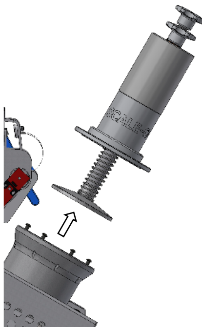
Figure 5: Measuring Cup Removal
