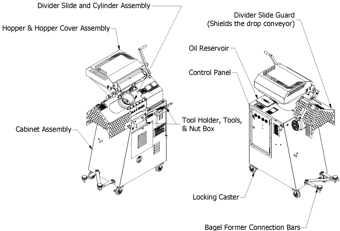
Figure 3: SAB Divider Overview
