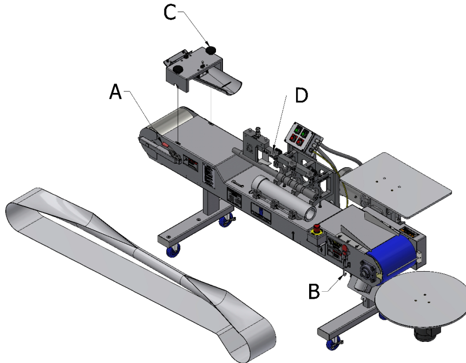
Figure 8: Belt Removal
