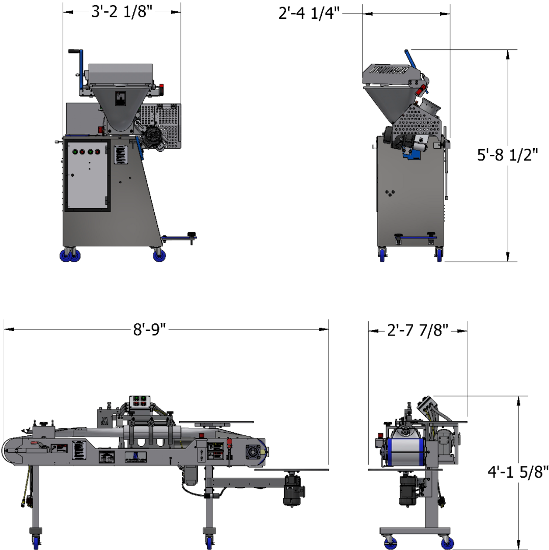
Figure 1: Specifications
