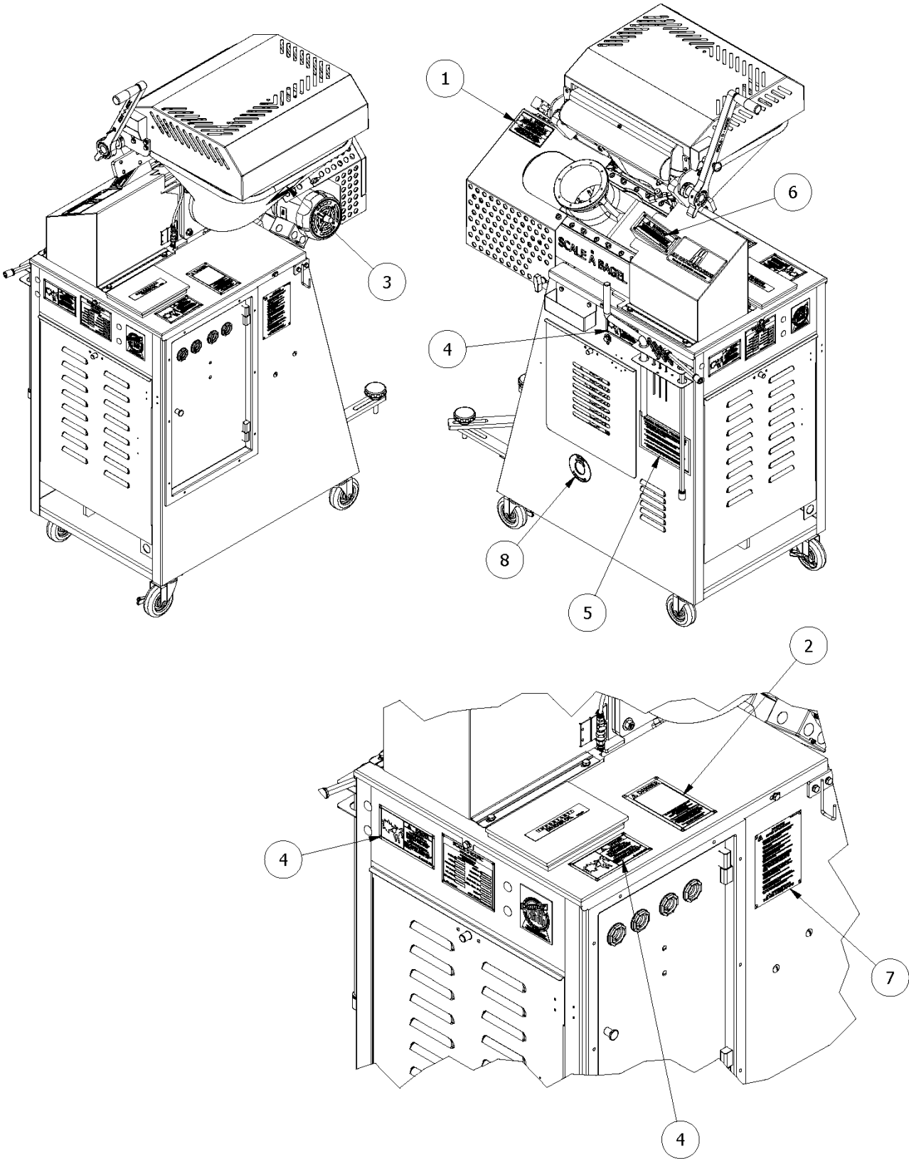
Figure 2: Warning Label Locations
