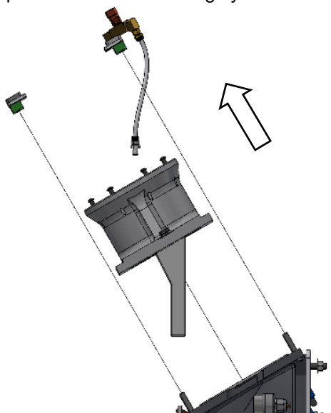
Figure 6: Divider Slide Removal
